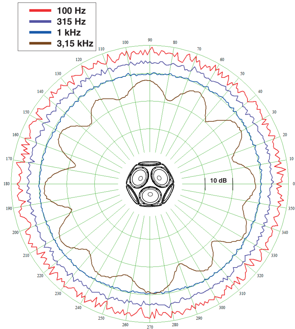
Sound power in different directions for Nor276. The measurement is done in a horizontal plane through the centre of the loudspeaker. The graph shows the responses for a sinusoidal signal at 100 Hz, 315 Hz, 1 kHz and 3,15 kHz.
