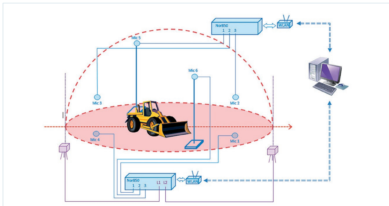
ISO 6395 setup
